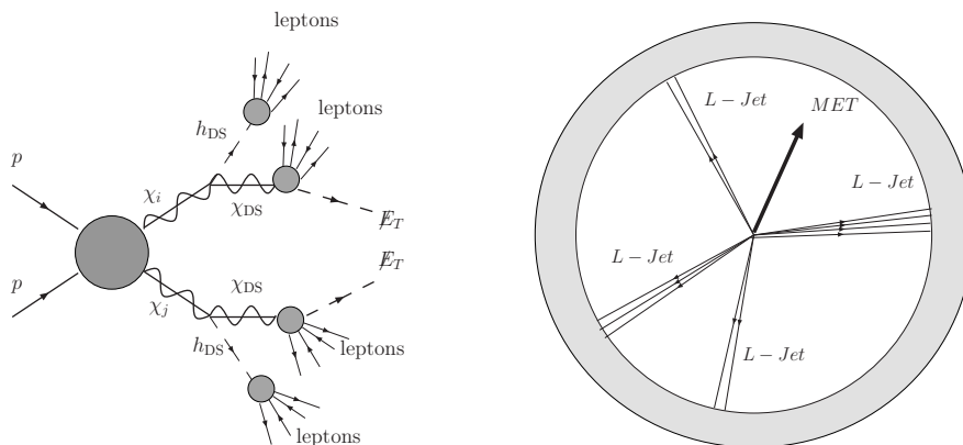
Figure 22. Pair-production of the SM LSP can result in spectacular lepton jet + MET events. On the left we depict the event topology. On the right we show a schematic representation of the resulting geometry.
