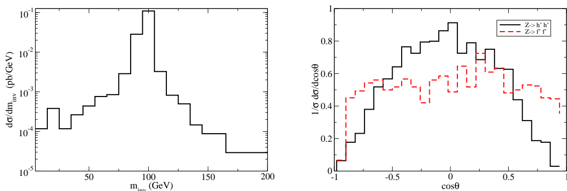
Figure 18. Left: Reconstructed Z^0 boson. Right: Normalized lepton jet angular distribution in the Z^0 boson's rest-frame.
