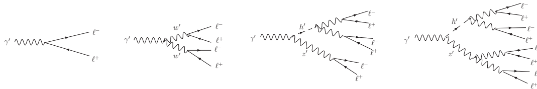
Figure 9. Typical decay chains starting with a dark gauge boson, labelled \gamma' in this plot. The dark decay chain can have several stages and involve additional dark sector states, such as other dark gauge bosons (labeled w', z' in this figure), and dark Higgses (labelled h' ).
