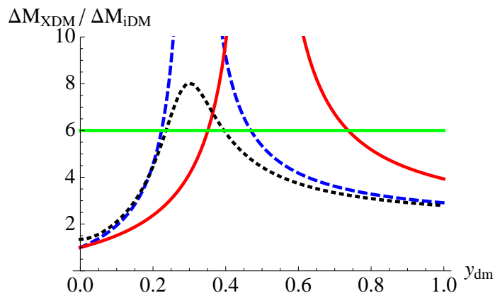
Figure 2. The ratio of the XDM splitting to the iDM splitting as a function of triplet dark matter U(1)_y hypercharge. The green horizontal line indicates the minimum ratio for simultaneously achieving both splittings. Red (line) is an example of two Higgs doublets with charge preserved, blue (dashed) represents two Higgs doublets with charge broken, and black (dots) adds a Higgs triplet to the previous case. For this example, the gauge couplings are g = 0.97 and g_y = 0.26 , and in terms of eq. (2.3) we have for all three models v_1 = 0.9 GeV, v_2 = 1.1 GeV and \lambda_{1,2,3,4} = 1 . Red (line) and black (dots) add charge breaking with \cos \alpha = 0.75 , and for black (dots), in terms of eq. (2.6), \lambda_\Phi = 1 , v_\Phi = 1 GeV and the triplet is decoupled from the doublets at tree-level by imposing the discrete symmetry: \Phi \rightarrow -\Phi .
