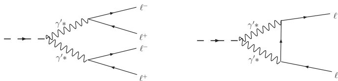
Figure 10. Two possible decay channels if the lightest dark sector state is a scalar from the dark Higgs sector.
