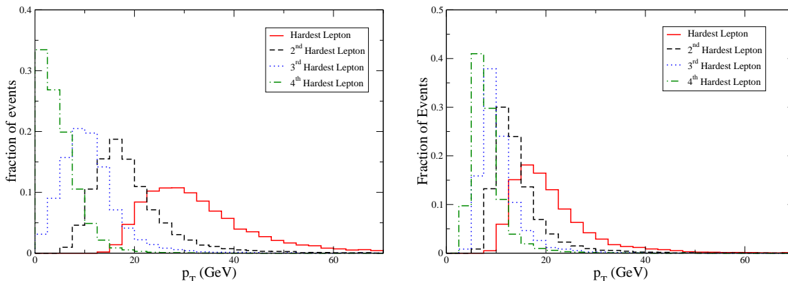
Figure 13. p_T distributions for cascades resulting in 4 (left) and 8 (right) leptons, for events with p_T > 50 GeV for \gamma' .
