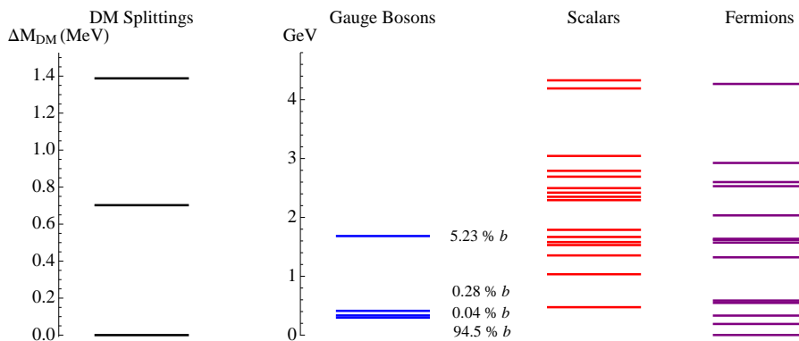
Figure 7. The spectrum of SUSY 1 , our two doublet and two complex triplet SUSY benchmark with kinetic mixing mediation. The left side displays the radiative mass splittings of the dark matter triplet, measured from the ground state. The larger splitting allows for the XDM explanation of INTEGRAL, but the smaller splitting is too large to explain DAMA with iDM. The right side shows the dark sector spectrum, and the b fractions of the gauge bosons are indicated. The triplet vevs break custodial symmetry, and all four gauge boson mass eigenstates are part b at tree-level. The gauginos and Higgsinos are strongly mixed after dark symmetry breaking. The lightest fermion, with mass \sim 2 MeV, is mostly gaugino and light because gauginos get no soft masses from kinetic mixing mediation. The second lightest fermion has a 3-body decay to the lightest fermion and a SM lepton pair, which can account for astrophysical lepton production and lead to a visibly displaced vertex at colliders.
