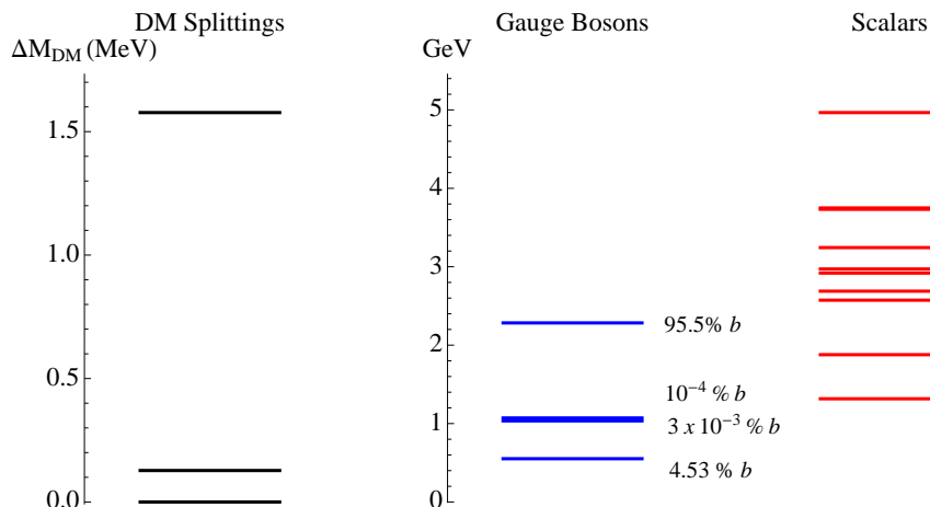
Figure 6. The spectrum of Non-SUSY 2 , our two doublet and one complex triplet non-SUSY benchmark. The left side displays the radiative mass splittings of the dark matter triplet, measured from the ground state. The splittings can account for the XDM and iDM explanations of INTEGRAL and DAMA, respectively. The right side shows the dark sector spectrum, and the b fractions of the gauge bosons are indicated. The triplet vev breaks custodial SU(2) , and all 4 gauge boson mass eigenstates mix with the b at tree-level, although for this example most of the b is contained in two of the mass eigenstates. The parameters of this benchmark are listed in the text.
