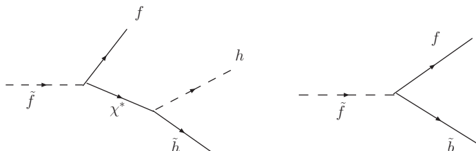
Figure 20. Decay of sfermion LSP.
