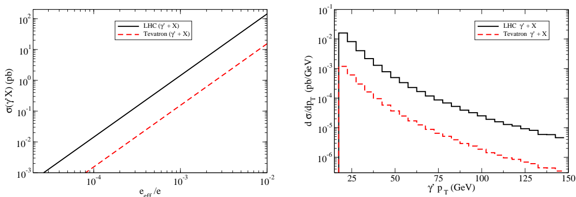
Figure 12. In the left pane, we show the rate of direct production of the dark gauge boson as a function of e_{\text{eff}}/e , where e_{\text{eff}} is the effective coupling of dark gauge boson to the Standard Model fields.
