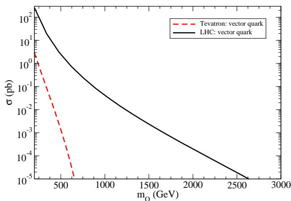
Figure 19. Production rate of one set of \mathbf{3} + \bar{\mathbf{3}} vector-like quarks, which can be part of the dark matter multiplet. The rate should be scaled by the number of such representations and the dimension of the dark matter representation under G_{\text{dark}} .
