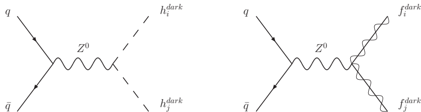
Figure 16. Z^0 production and two possible decay channels into the dark sector. On the left we depict a decay into the dark Higgs sector. Fermionic channels, such as the one shown on the right, are dominantly associated with the Higgsino states possible in supersymmetric versions of the model.
